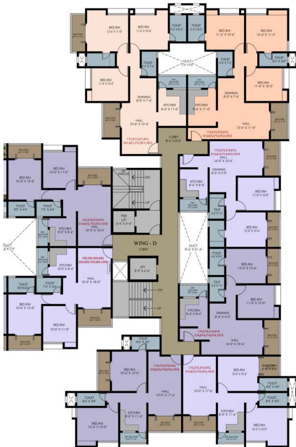
1st, 2nd, 3rd, 4th, 5th, 6th, 7th, 9th & 10th Floor Plan (BUILDING 3)
